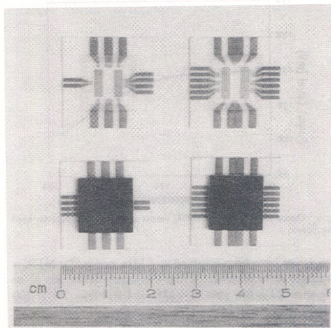
Fig. 5. Two versions of the ceramic pack ages shown with and without lids.
